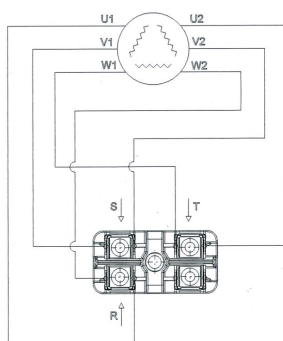
THREE-PHASE DELTA CONNECTION
