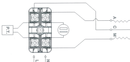
SINGLE PHASE CONNECTION AND CIRCUIT SWITCH PROTECTOR
