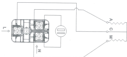
SINGLE PHASE CONNECTION
