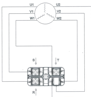
THREE-PHASE STAR CONNECTION
